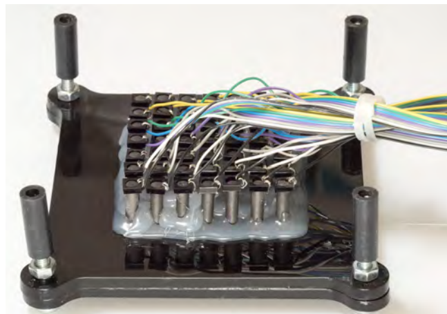
Figure 4. Back side view of 7x7 graphite electrode array display. Sealing between the graphite electrode rods and the acrylic substrate of the display is achieved through a silicone glue, which is NaOH-resistant. Each graphite rod is wired individually through a laser-cut acrylic adapter. The height and balance of the display table level is adjustable with respect to the ground by rotating the screws of the four supporting legs.
