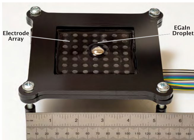
Figure 3. The 7x7 graphite electrode array display used in this study (top view). The figure also highlights the size of the EGaln blob using during the experiments (9 grams).
